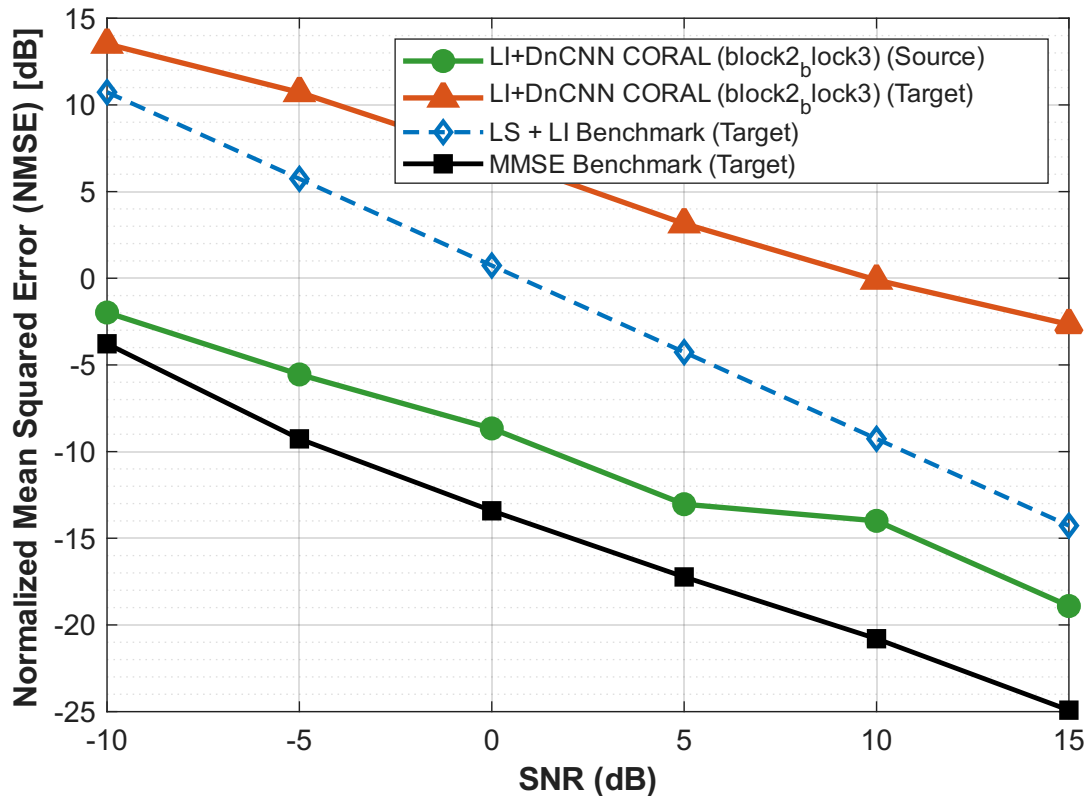
NMSE (dB): Source vs Target Domain Adaptation (LI+DnCNN CORAL (block 2 b lock3))
