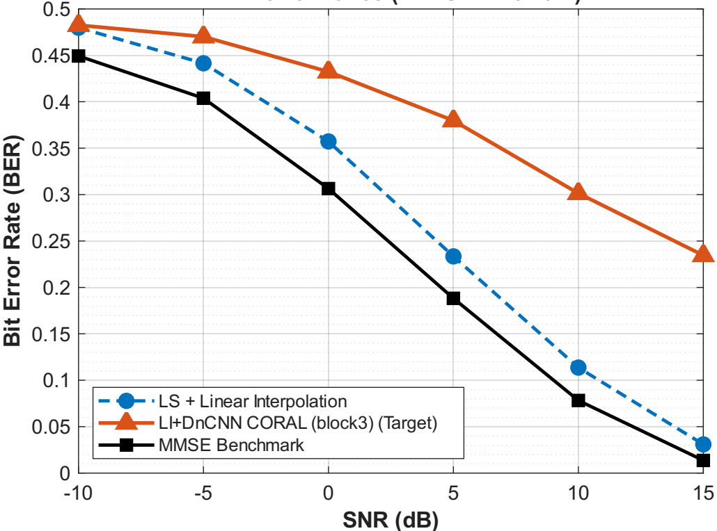
BER Performance (TARGET Domain)
