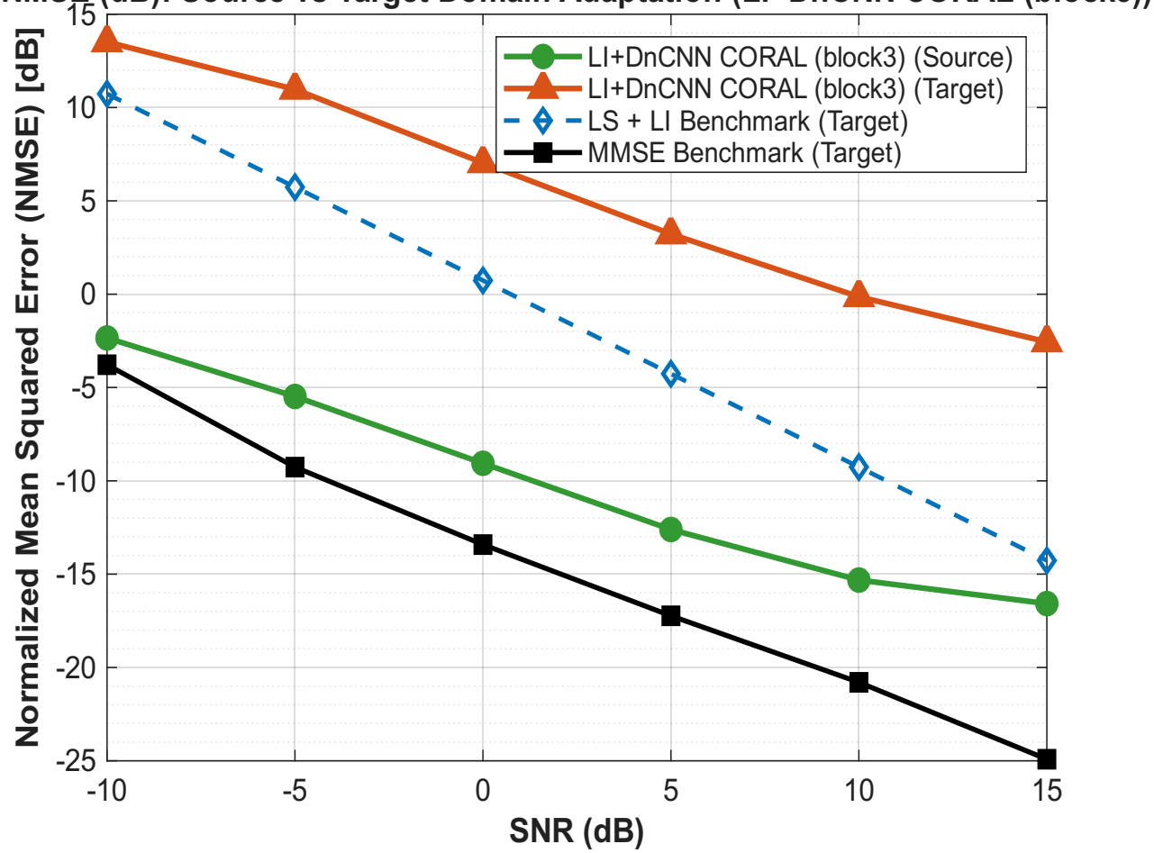
NMSE (dB): Source vs Target Domain Adaptation (LI+DnCNN CORAL (block3))
