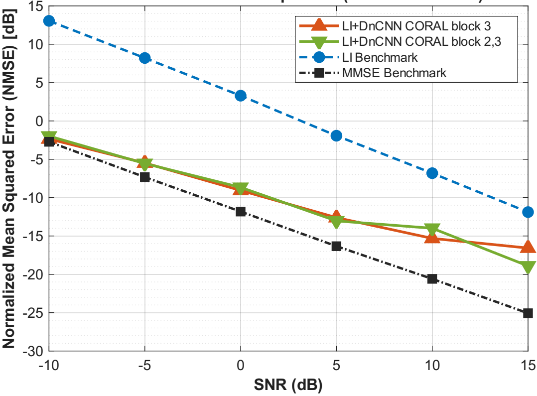
NMSE Performance Comparison (SOURCE Domain)
