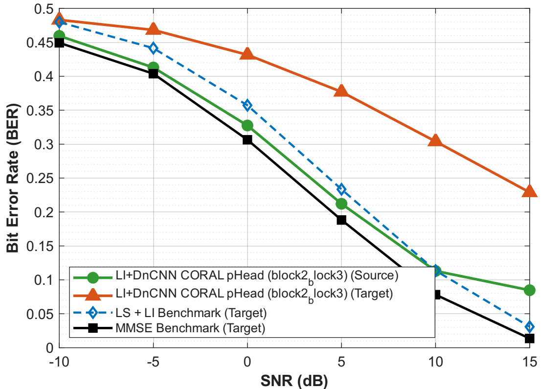
BER: Source vs Target Domain Adaptation (LI+DnCNN CORAL pHead (block 2_b lock3))
