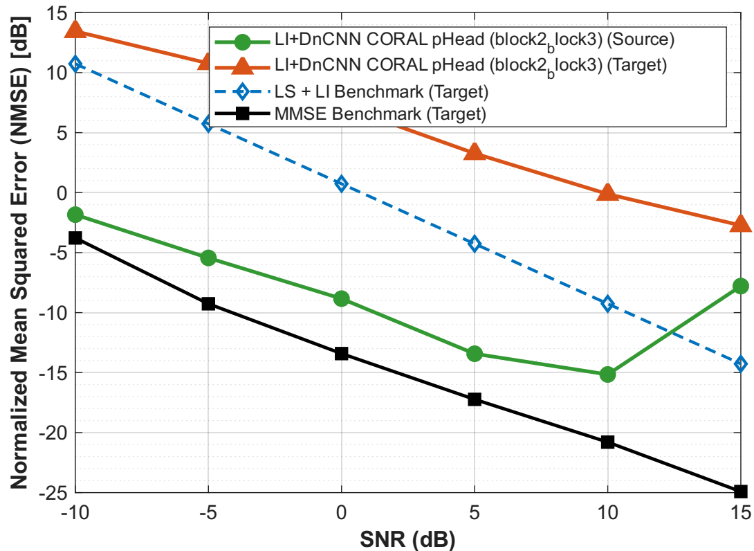
NMSE (dB): Source vs Target Domain Adaptation (LI+DnCNN CORAL pHead (block2 b lock3))
