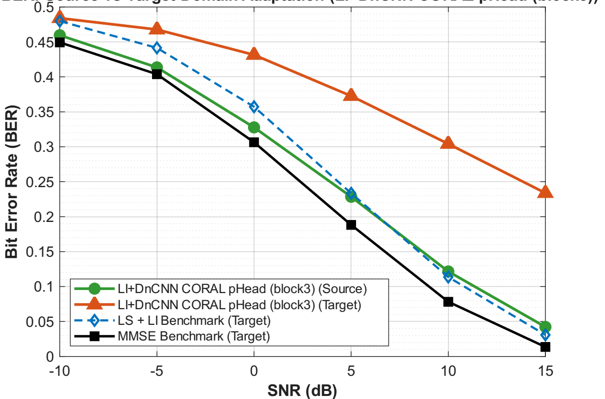
BER: Source vs Target Domain Adaptation (LI+DnCNN CORAL pHead (block3))
