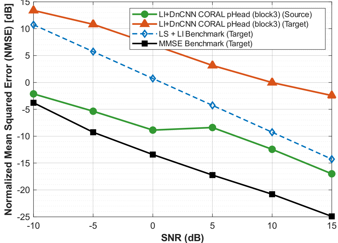
NMSE (dB): Source vs Target Domain Adaptation (LI+DnCNN CORAL pHead (block3))
