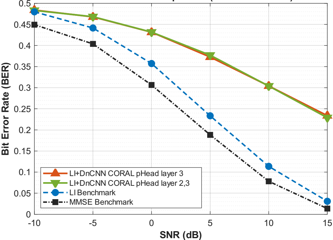
BER Performance Comparison (TARGET Domain)
