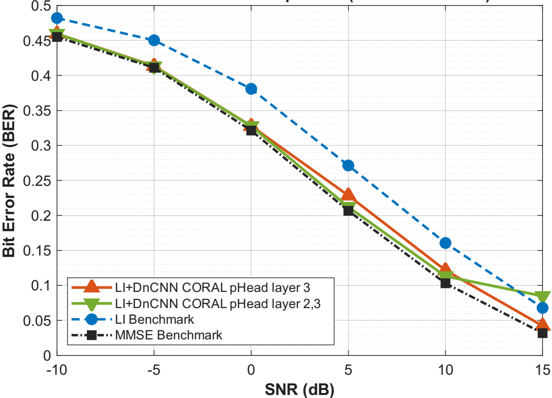
BER Performance Comparison (SOURCE Domain)
