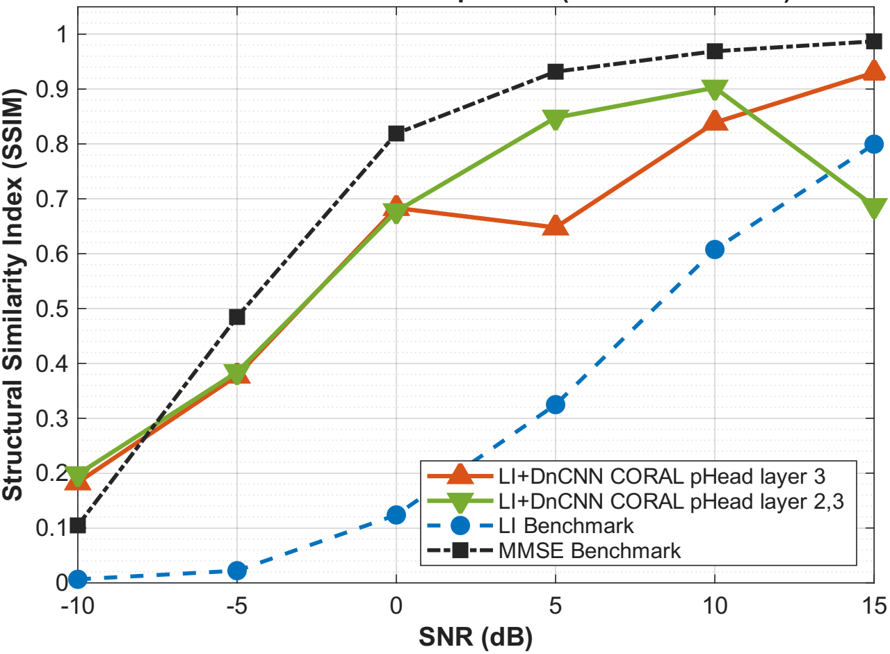
SSIM Performance Comparison (SOURCE Domain)
