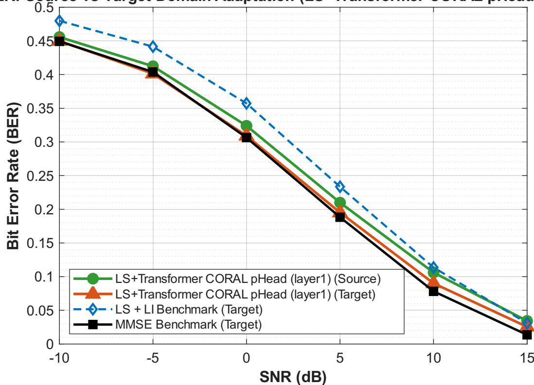
BER: Source vs Target Domain Adaptation (LS+Transformer CORAL pHead (layer1))
