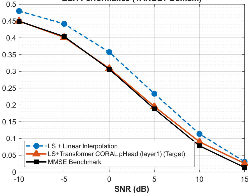
BER Performance (TARGET Domain)
