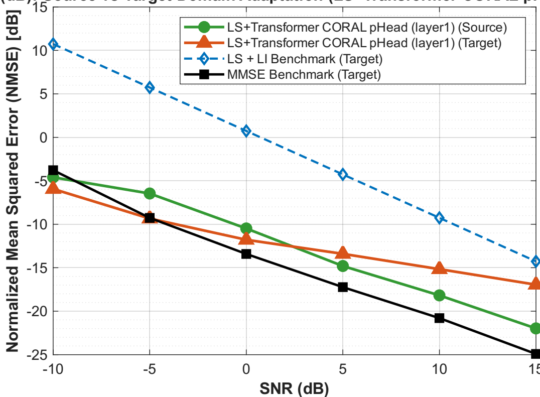
NMSE (dB): Source vs Target Domain Adaptation (LS+Transformer CORAL pHead (layer1))
