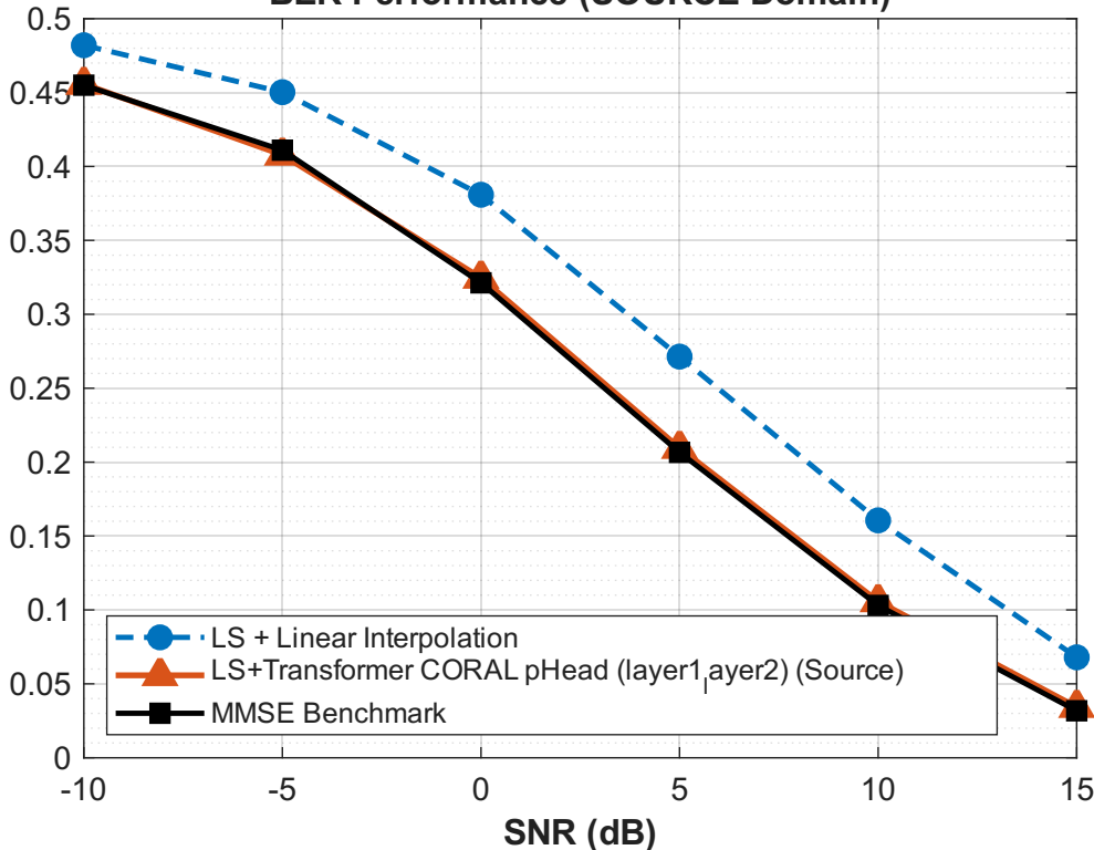
BER Performance (SOURCE Domain)
