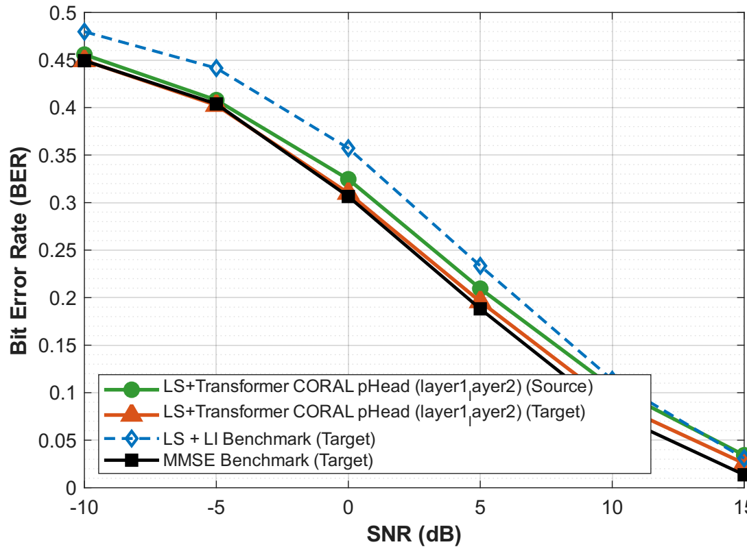
BER: Source vs Target Domain Adaptation (LS+Transformer CORAL pHead (layer1ayer2))
