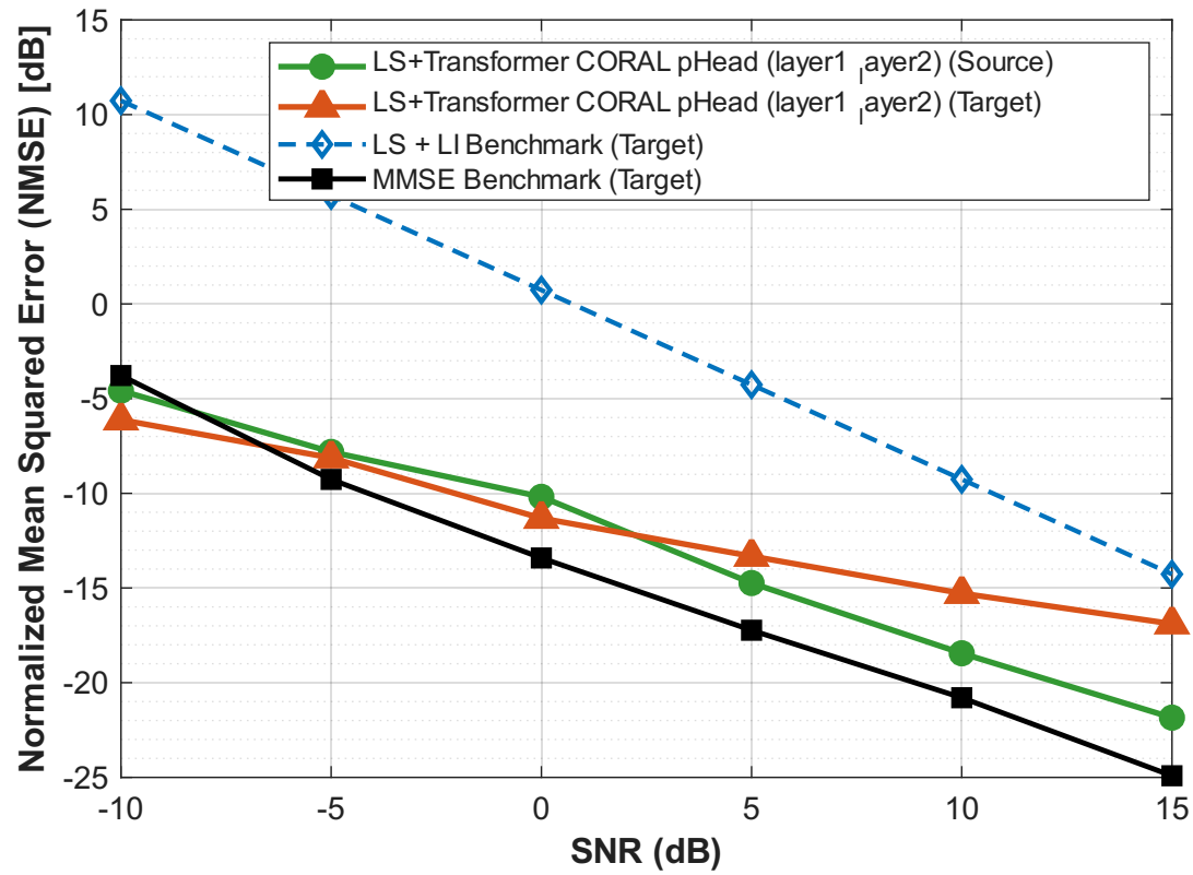
NMSE (dB): Source vs Target Domain Adaptation (LS+Transformer CORAL pHead (layer1ayer2))
