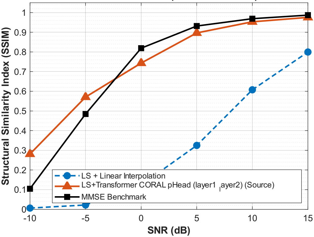
SSIM Performance (SOURCE Domain)
