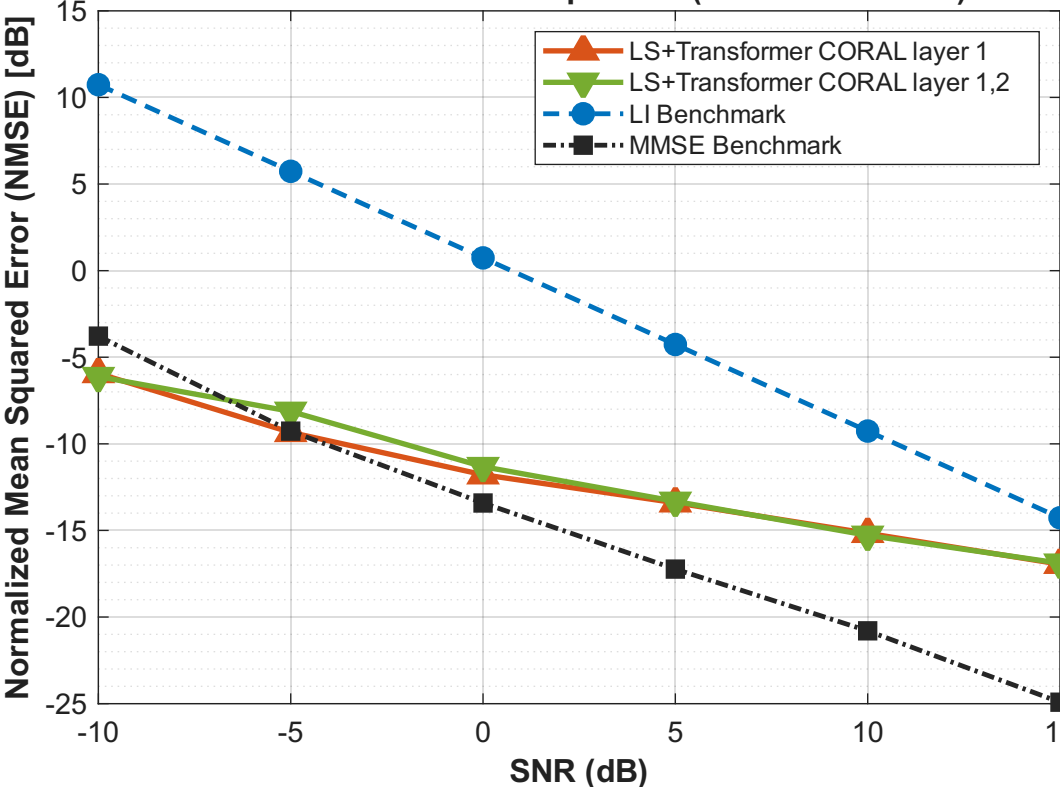
NMSE Performance Comparison (TARGET Domain)
