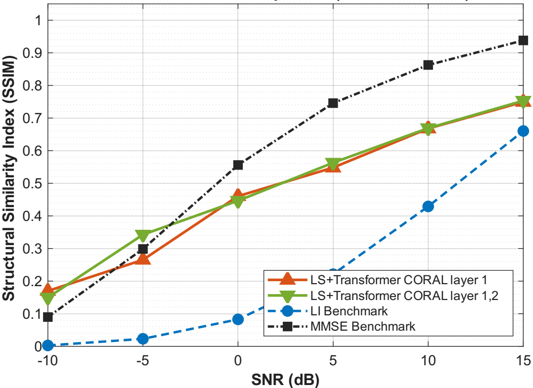
SSIM Performance Comparison (TARGET Domain)
