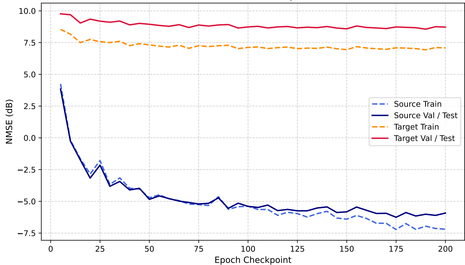
NMSE (dB) Across Epochs
