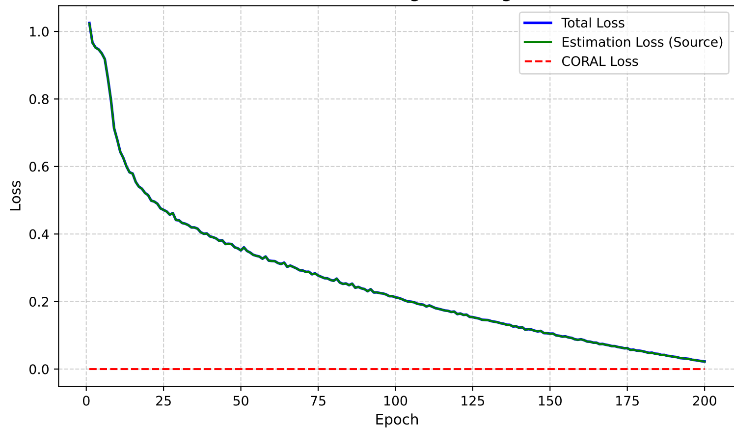
DnCNN CORAL Training Loss Progression
