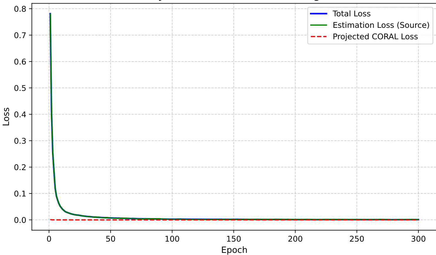
HA02 Projection-Head CORAL Loss Progression
