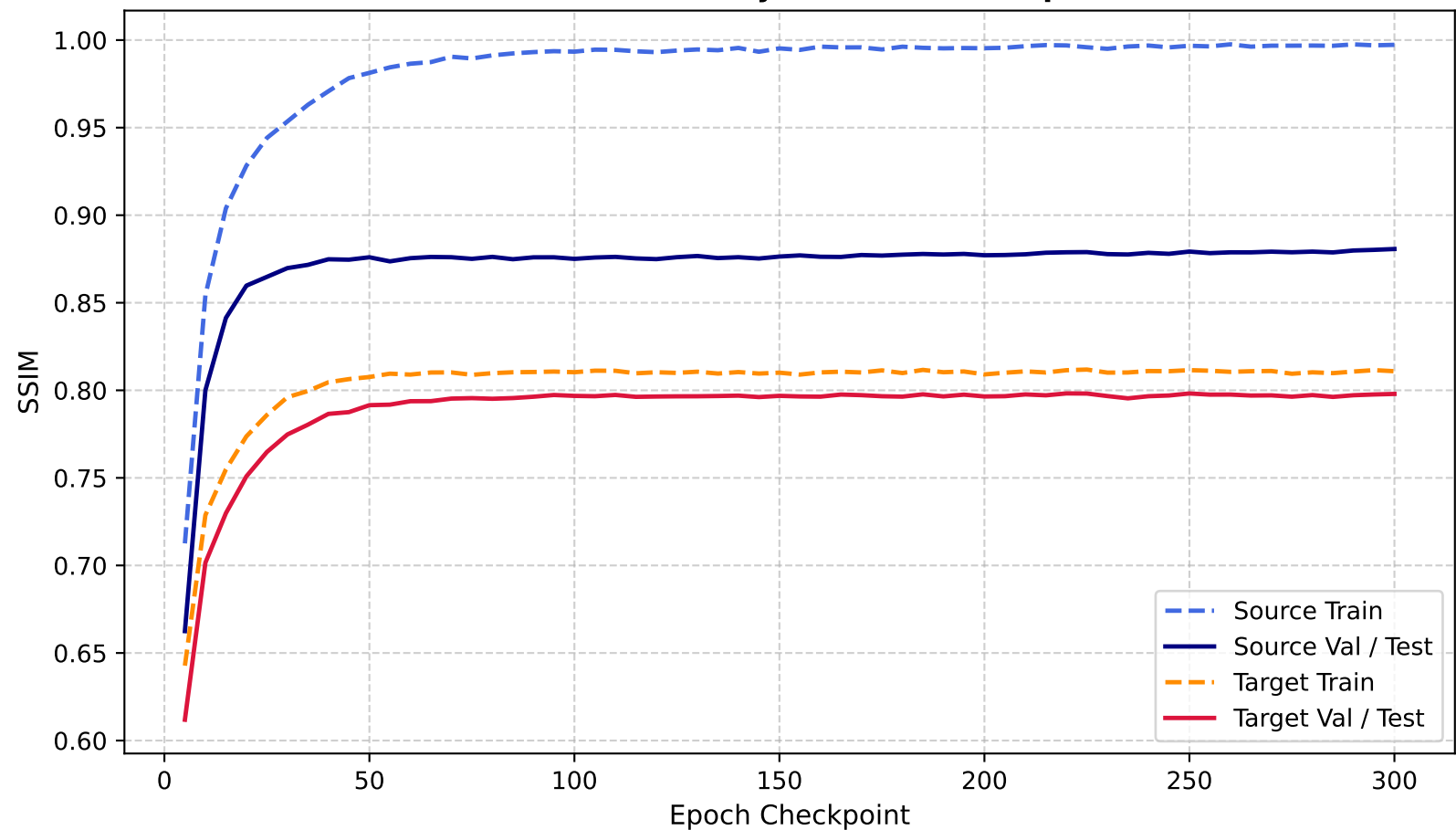
Structural Similarity (SSIM) Across Epochs
