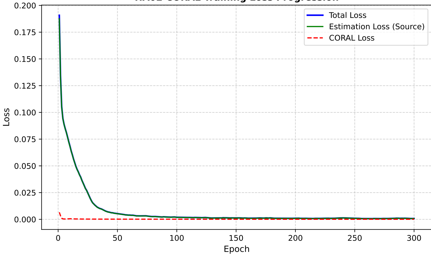
HA02 CORAL Training Loss Progression
