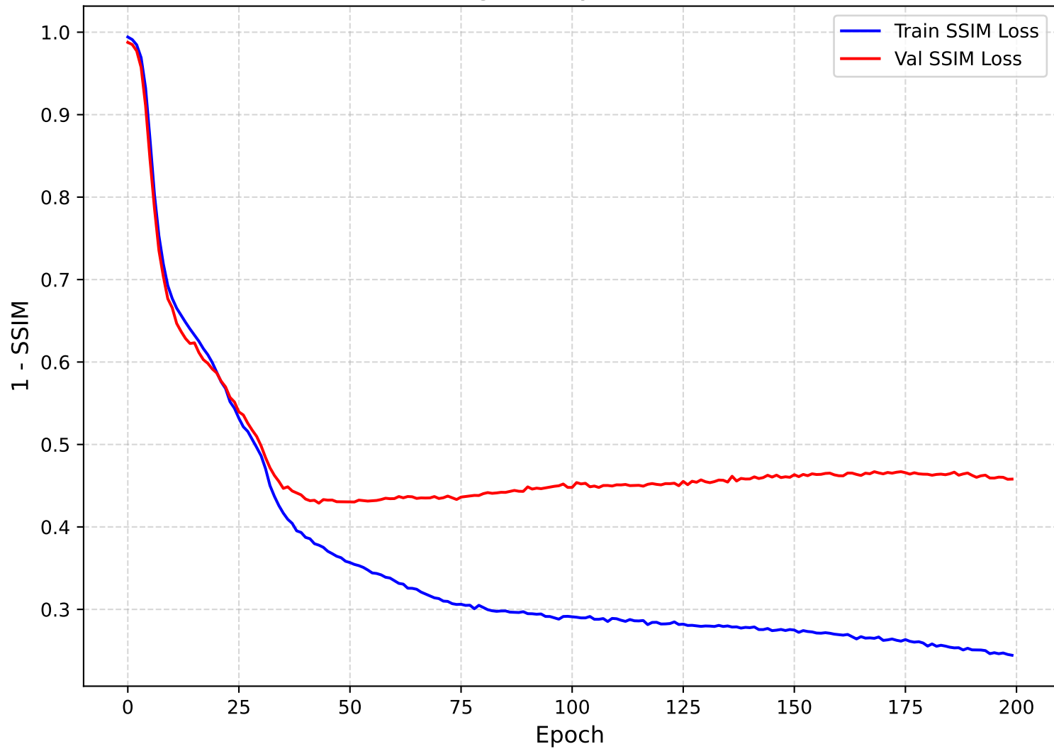
Training History - SSIM Loss
