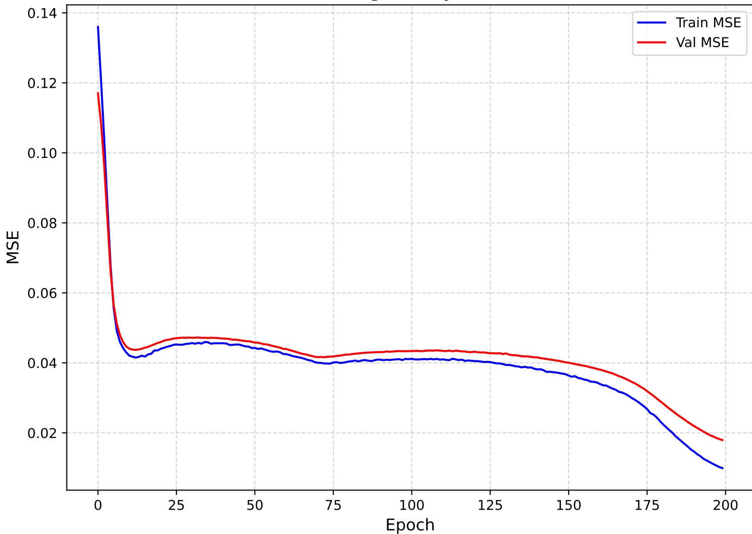
Training History - MSE
