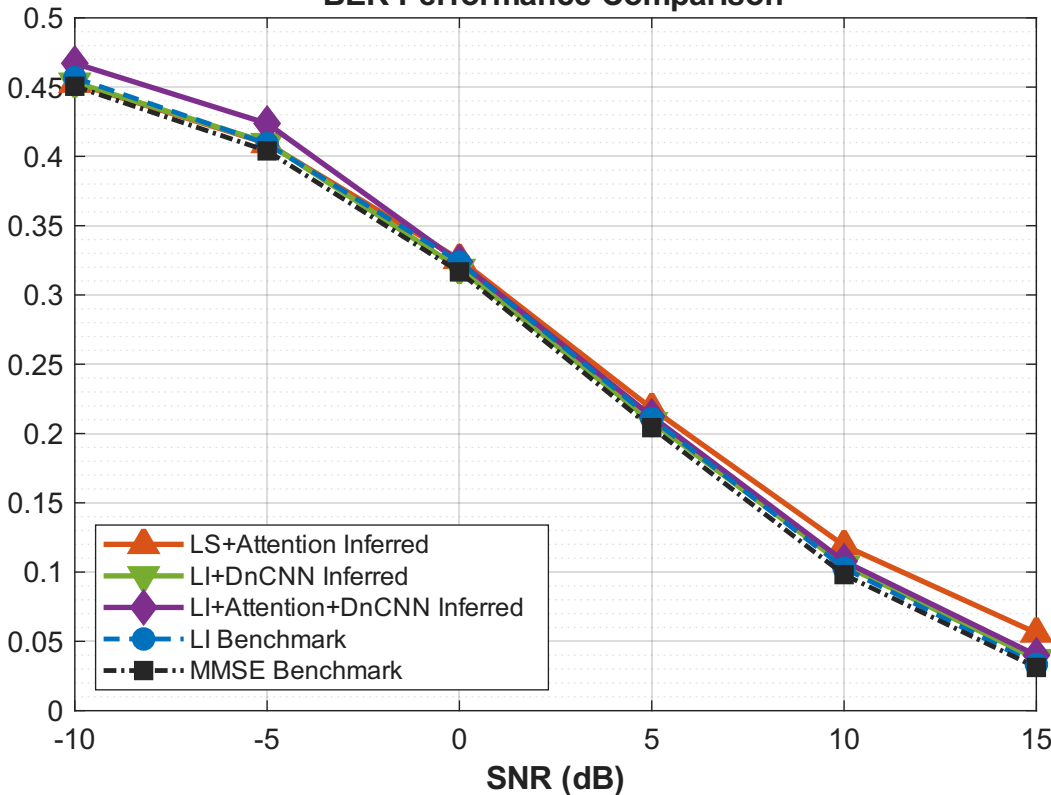
BER Performance Comparison
