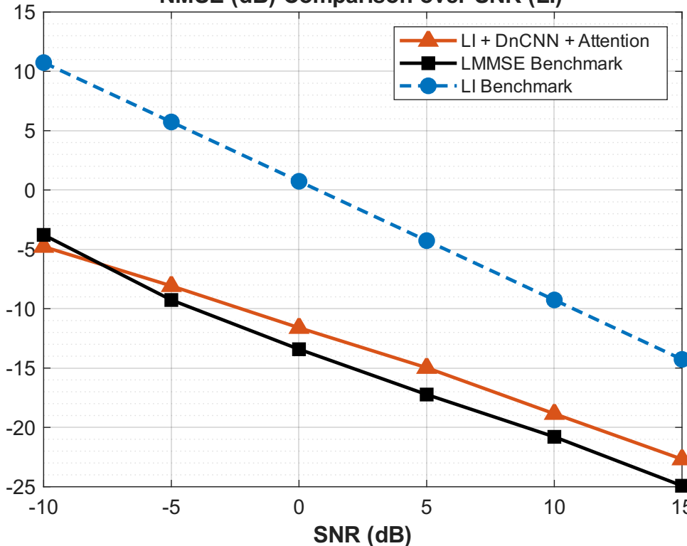
NMSE (dB) Comparison over SNR (LI)
