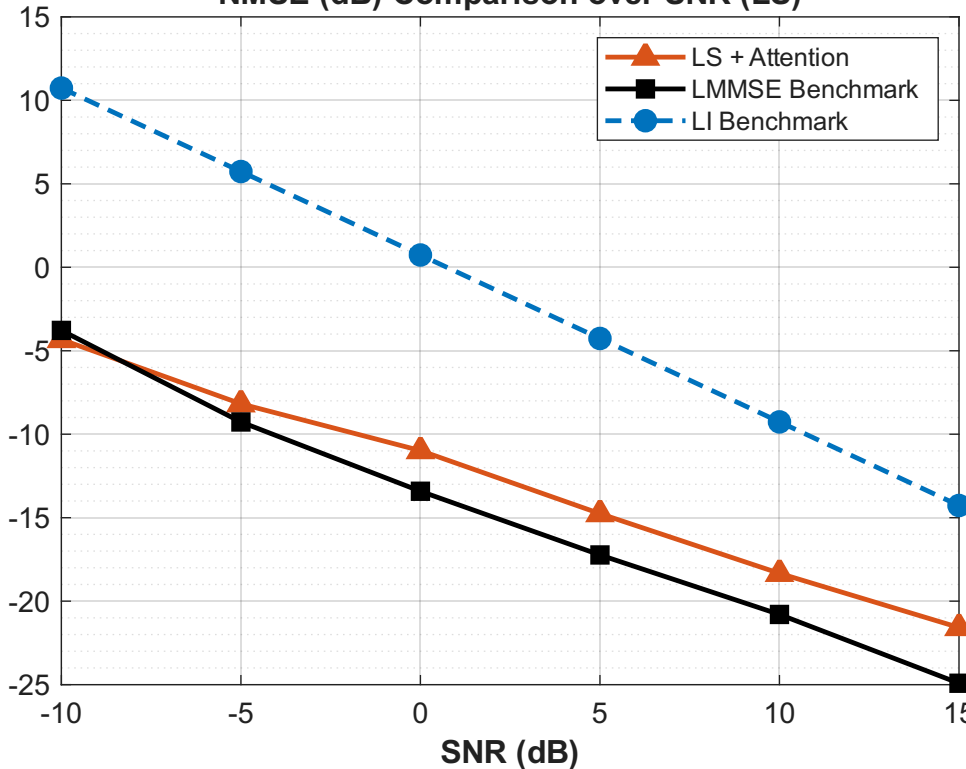
NMSE (dB) Comparison over SNR (LS)
