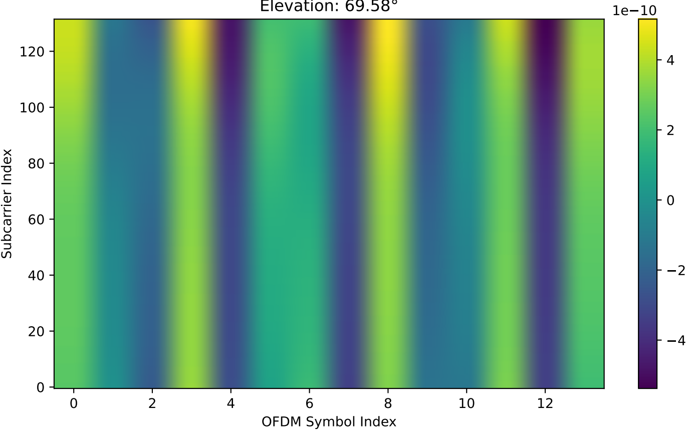
Original Perfect Channel (Full Doppler): Real Part of Channel 0 (DUR) Elevation: 69.58^\circ
