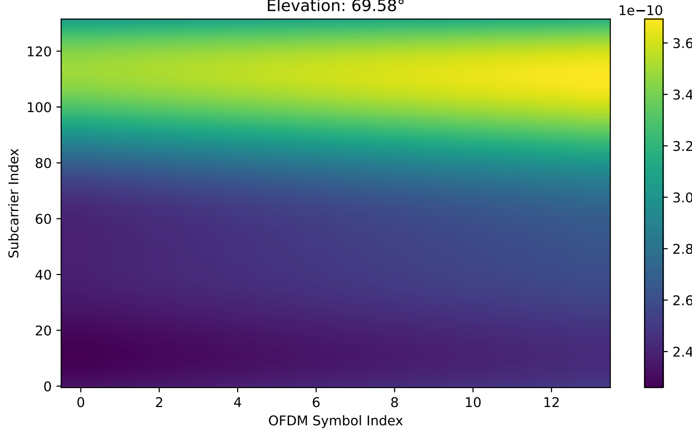
Effective Compensated Channel (Precompensated Satellite Doppler): Real Part of Channel 0 (DUR) Elevation: 69.58° 1e-10
