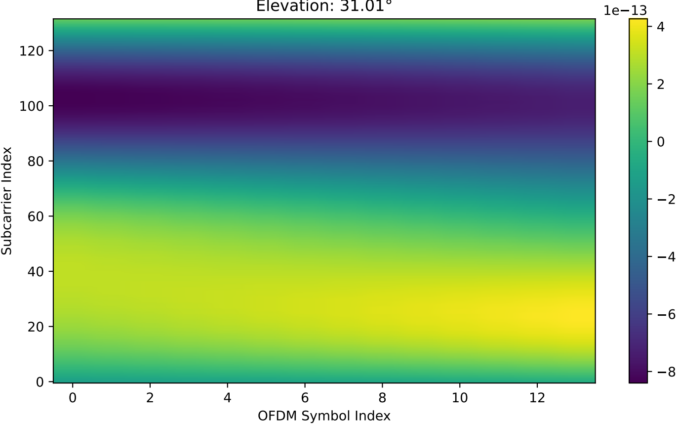
Original Perfect Channel (Full Doppler): Real Part of Channel 0 (DUR) Elevation: 31.01^\circ
