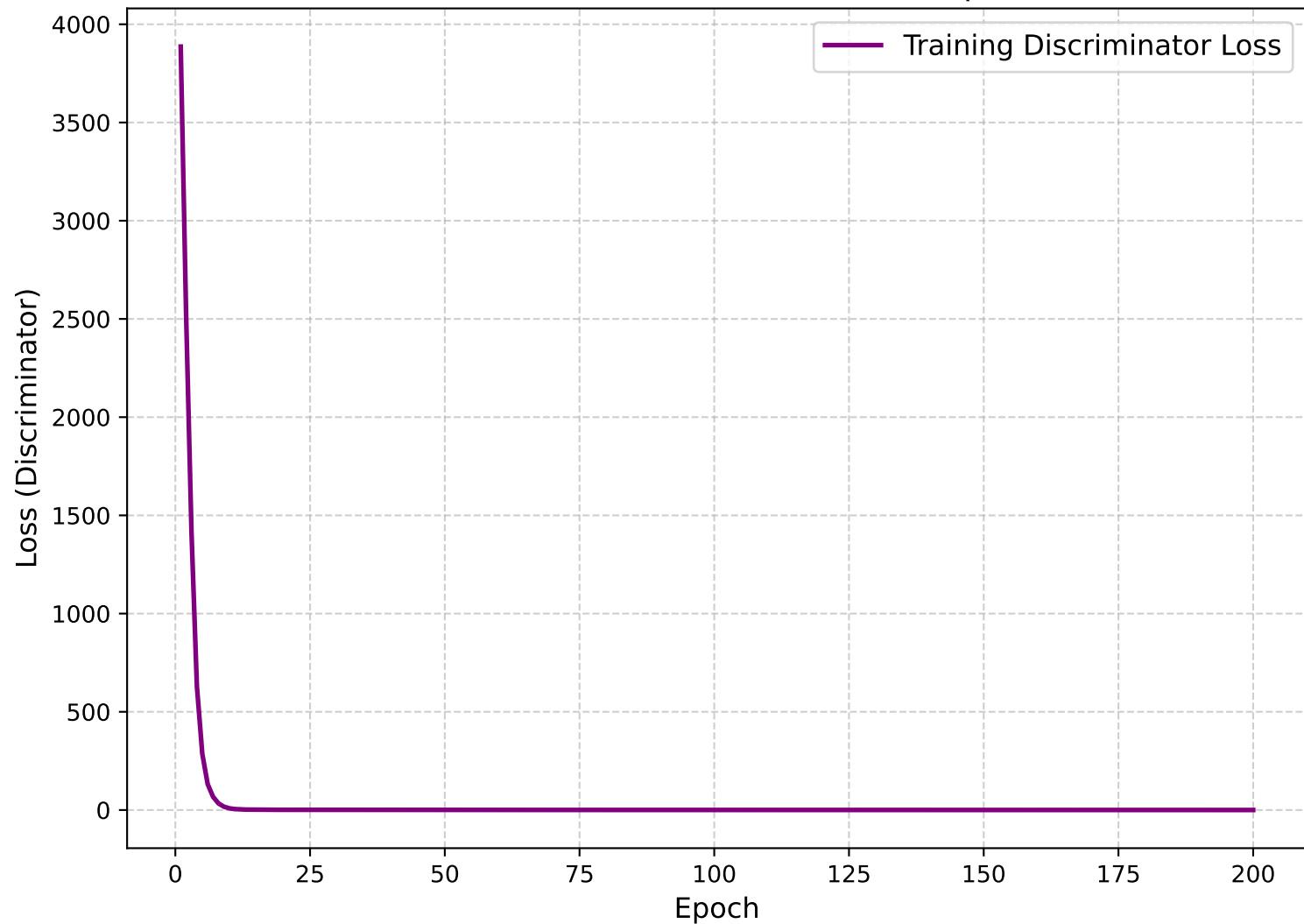
WGAN-GP Discriminator Loss over Epochs
