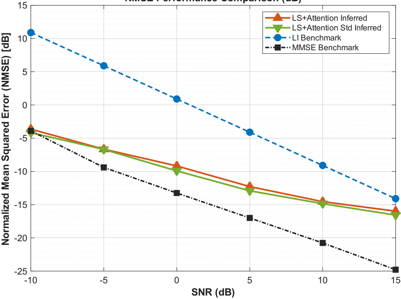
NMSE Performance Comparison (dB)
