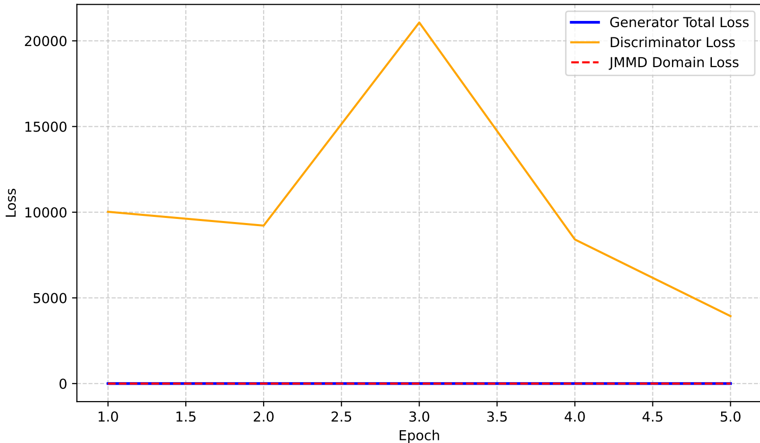
JMMD cGAN Training Loss Progression
