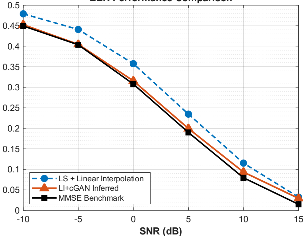
BER Performance Comparison
