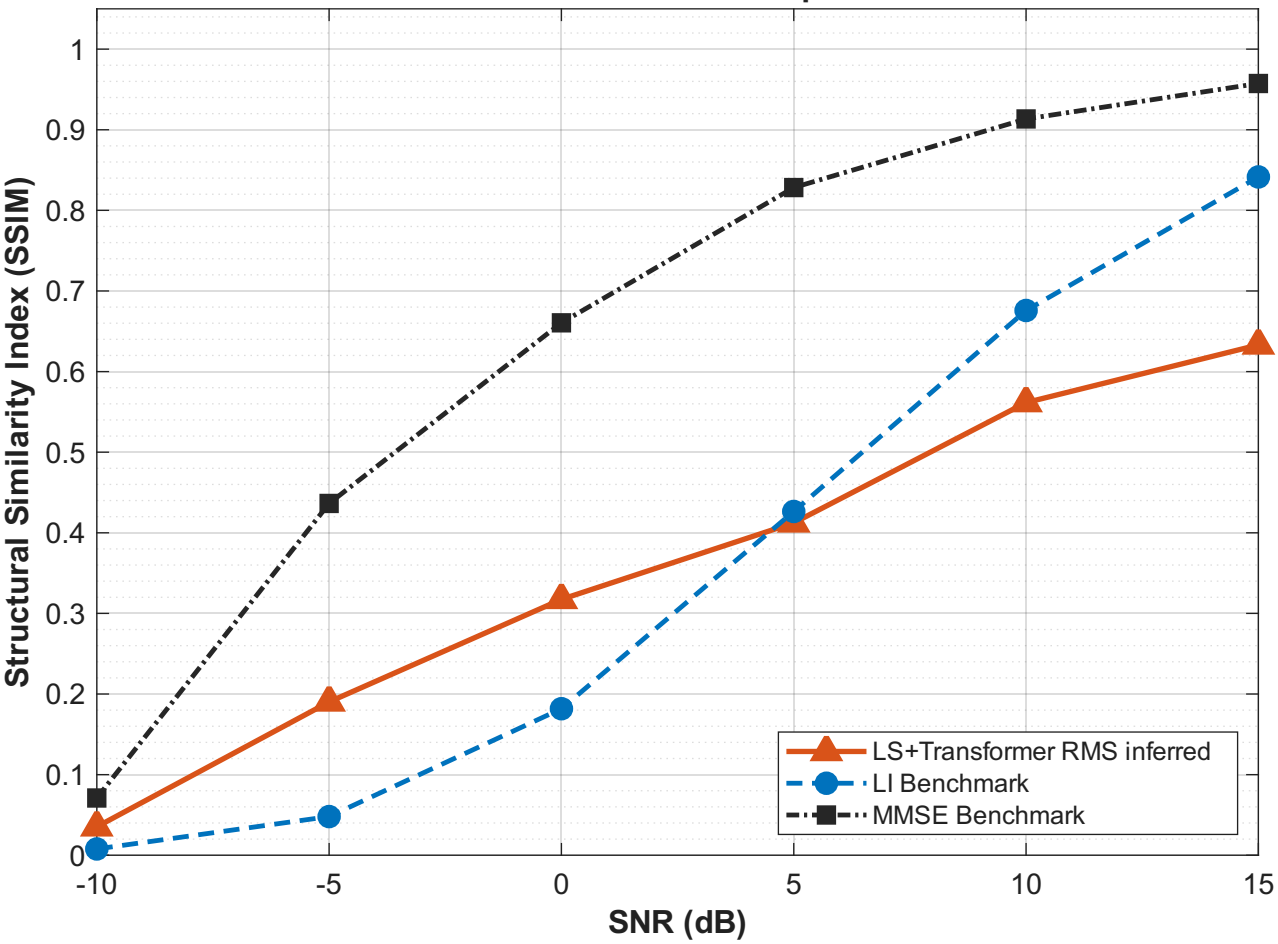
SSIM Performance Comparison
