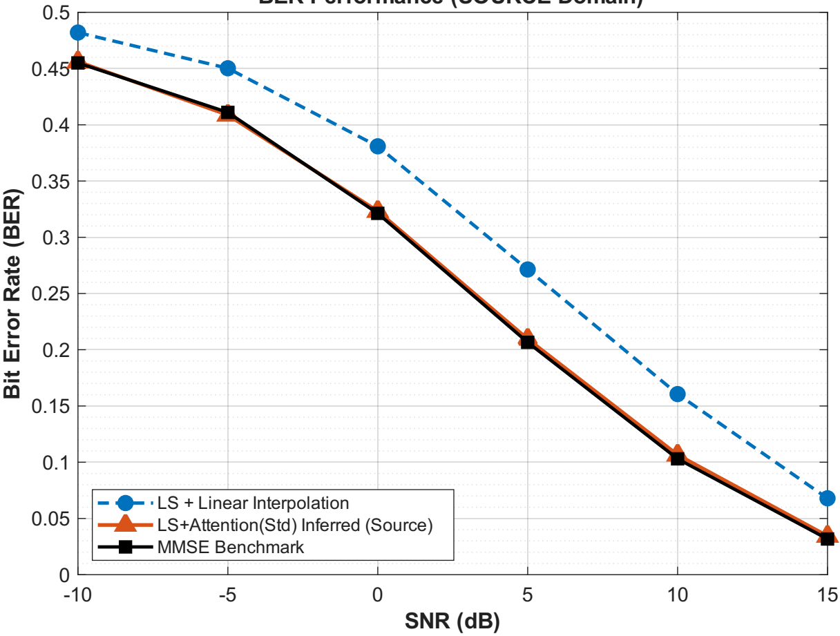
BER Performance (SOURCE Domain)
