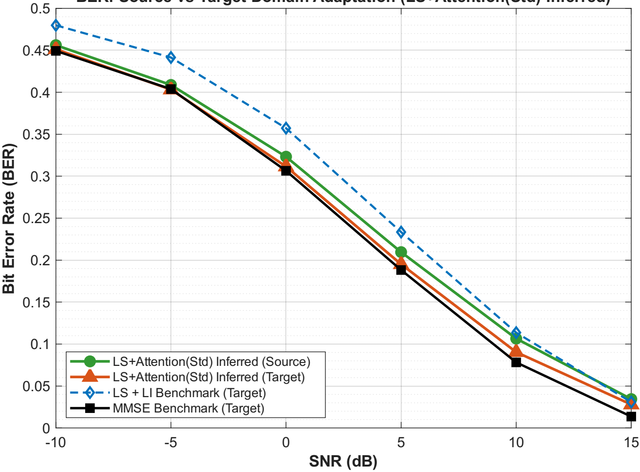
BER: Source vs Target Domain Adaptation (LS+Attention(Std) Inferred)
