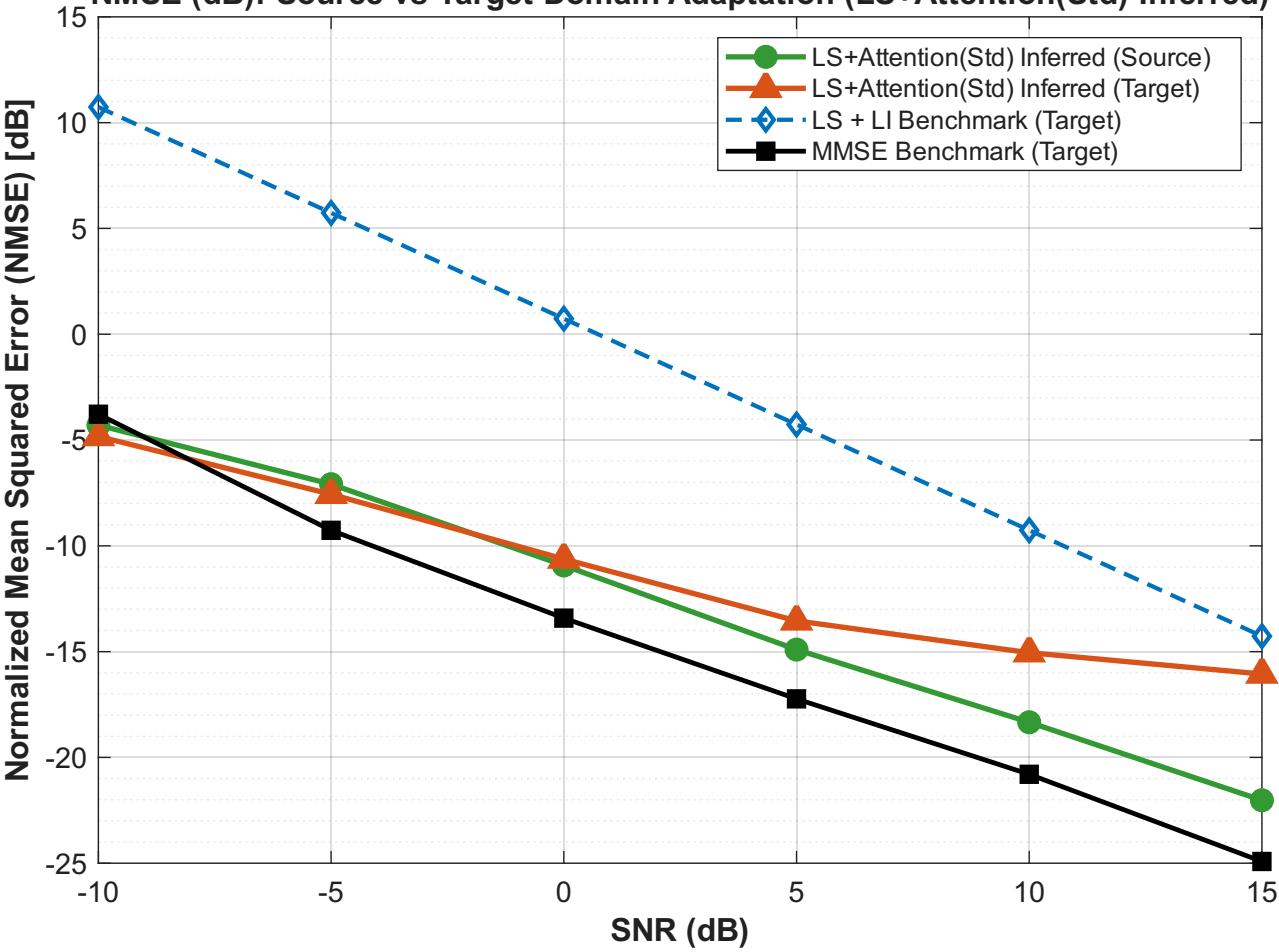
NMSE (dB): Source vs Target Domain Adaptation (LS+Attention(Std) Inferred)
