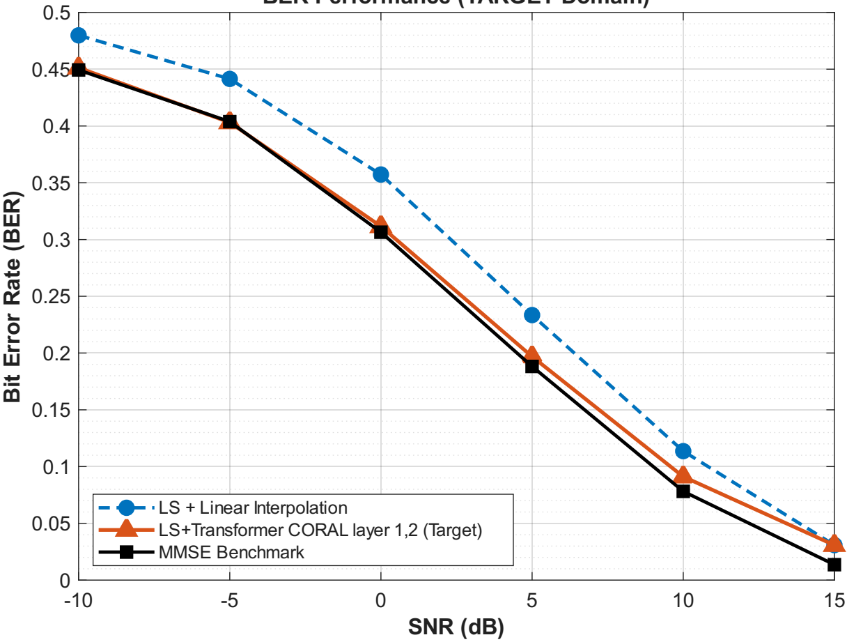
BER Performance (TARGET Domain)
