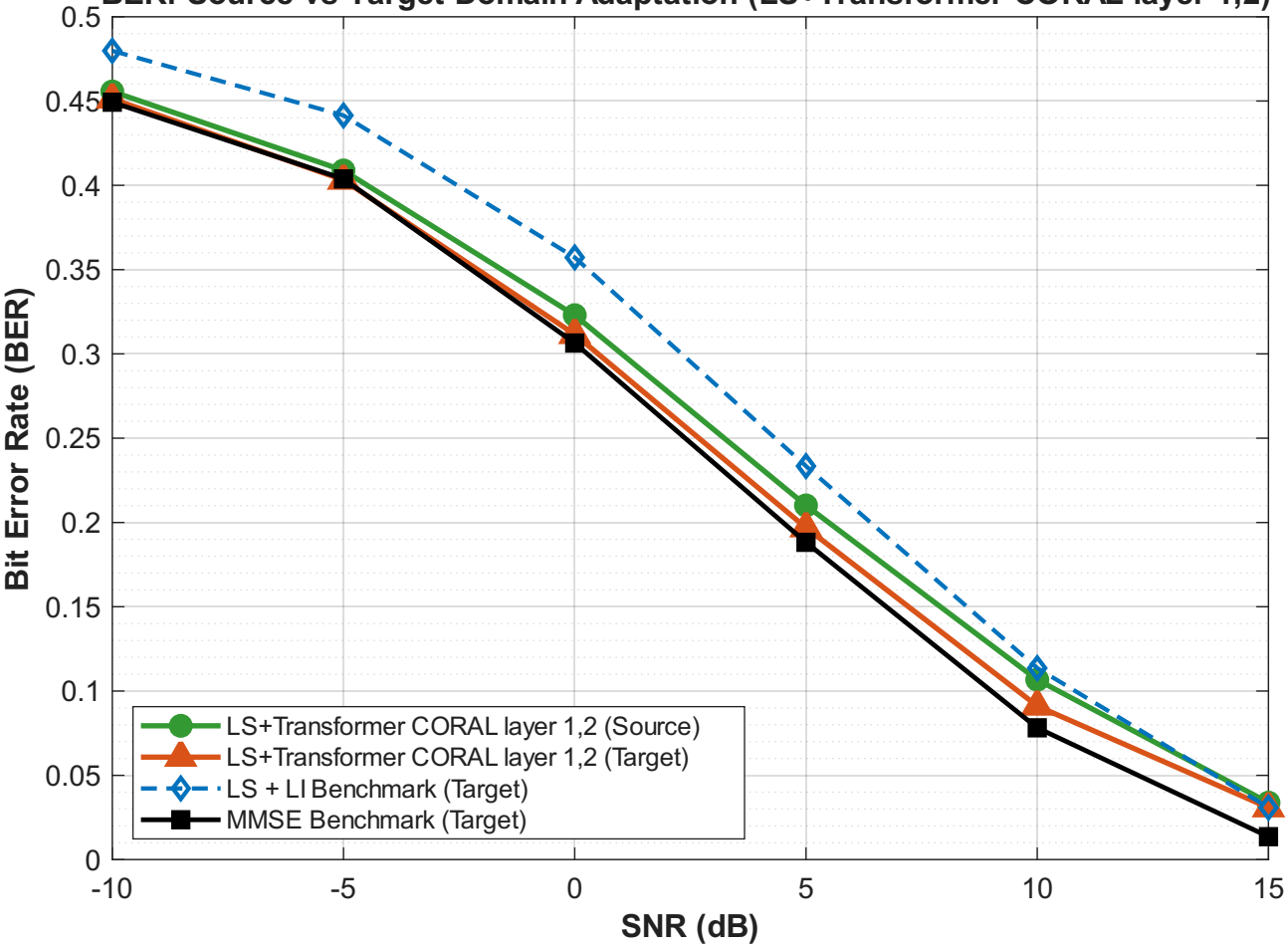
BER: Source vs Target Domain Adaptation (LS+Transformer CORAL layer 1,2)
