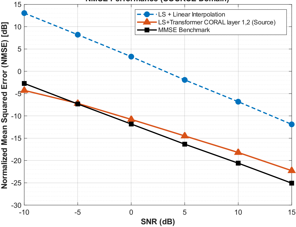
NMSE Performance (SOURCE Domain)
