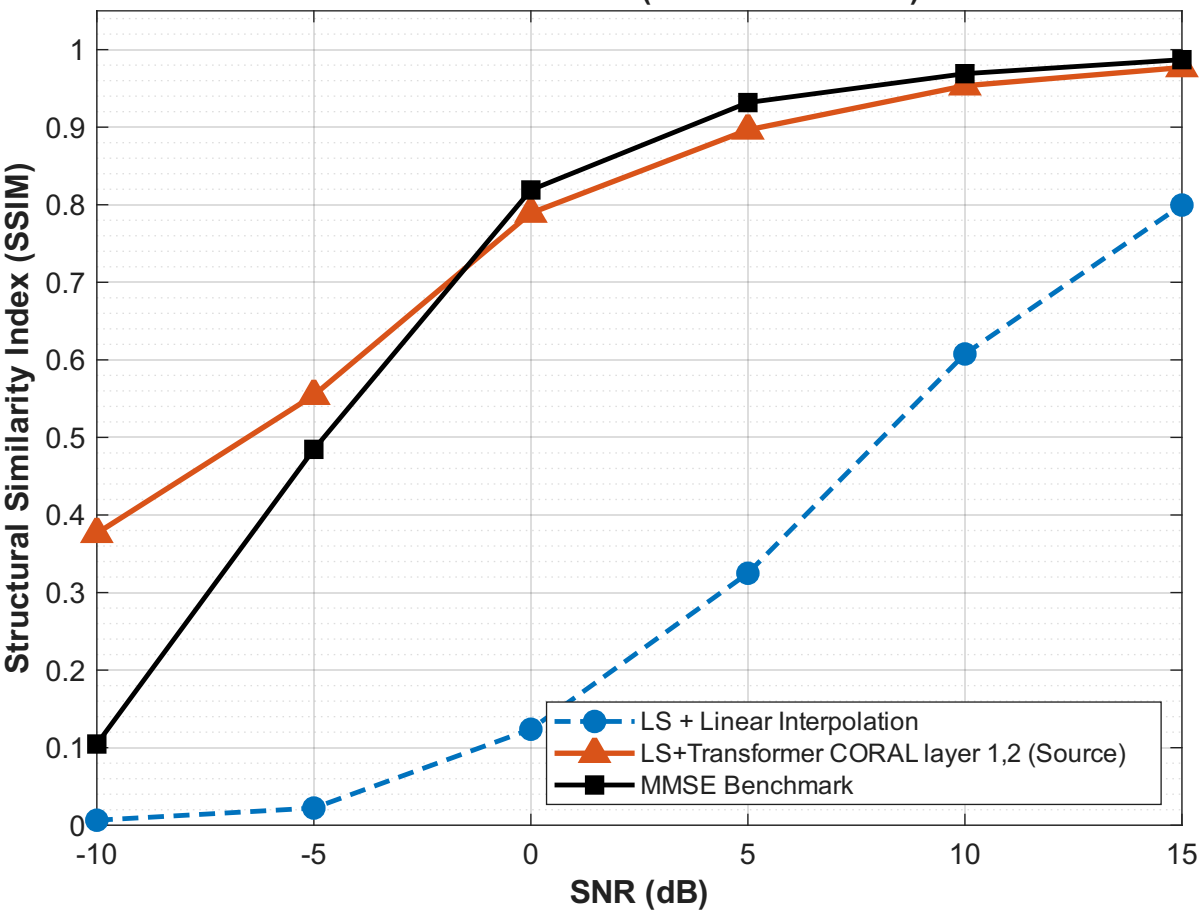
SSIM Performance (SOURCE Domain)
