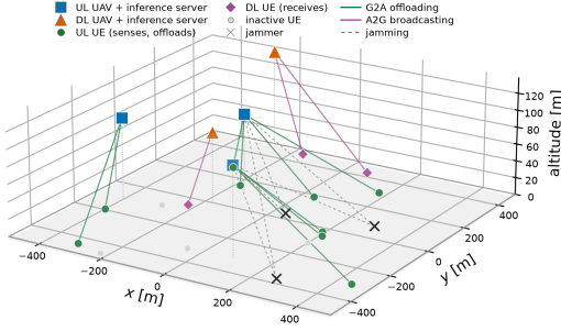
Fig. 1. One HPPP realisation of the SI-TNTN drawn by the simulator: UAVs hover at their sampled altitudes over ground UEs and jammers, with G2A offloading, A2G broadcasting, and jamming on both directions.
