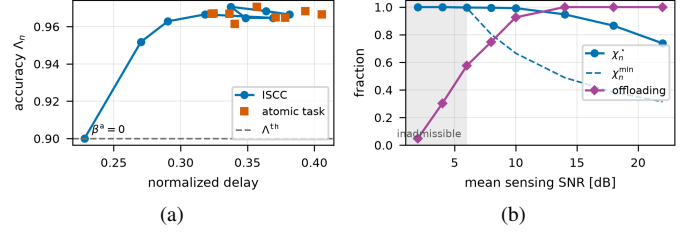
Fig. 4. ISCC effects: (a) accuracy–delay frontier swept over \beta^a , versus the atomic-task baseline; (b) optimal retention \chi_n^* , retention floor \chi_n^{min} , and fraction of offloading UEs versus mean sensing SNR.
