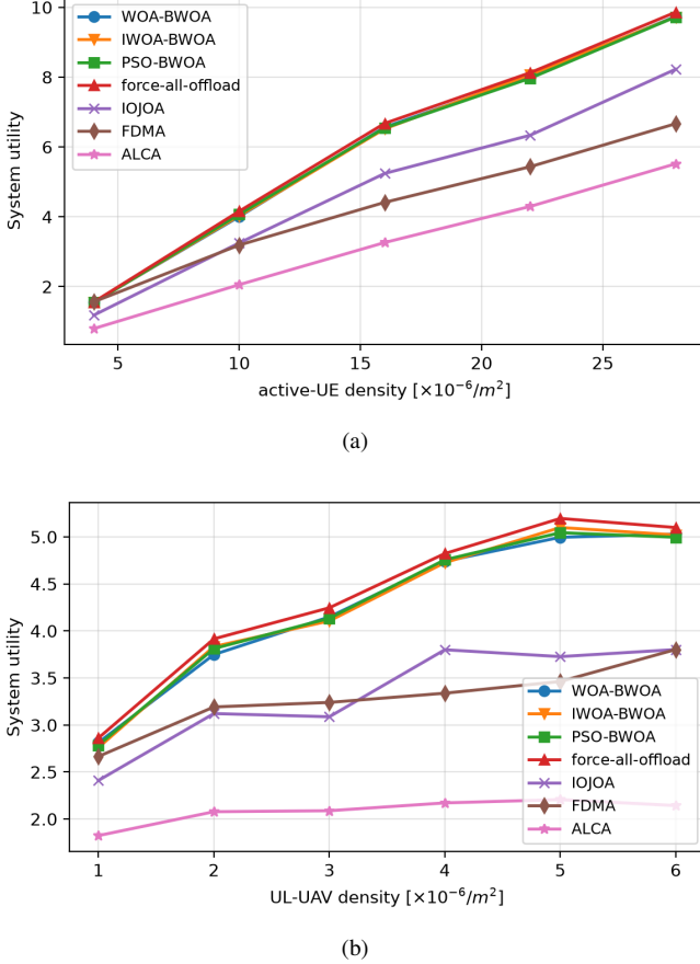
Fig. 3. (a) Utility versus active-UE density for WOA/IWOA/PSO-BWOA (MF-SIC), force-all-offload, IOJOA, FDMA, and ALCA. (b) Utility versus UL UAV-server density.
