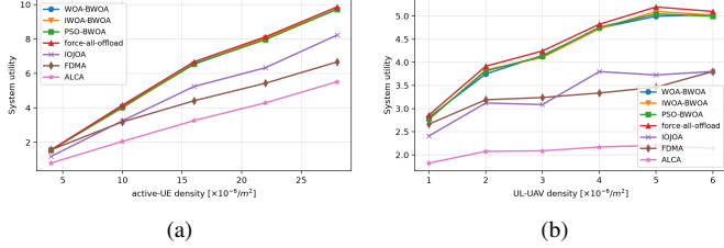
Fig. 3. (a) Utility versus active-UE density for WOA/IWOA/PSO-BWOA (MF-SIC), force-all-offload, IOJOA, FDMA, and ALCA. (b) Utility versus UL UAV-server density.
