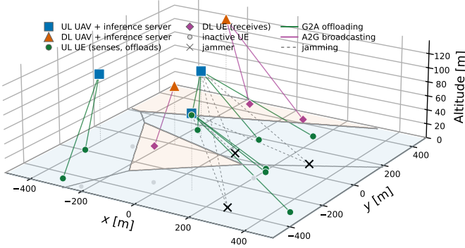
Fig. 1. One HPPP realisation of the SI-TNTN drawn by the simulator: UAVs hover at their sampled altitudes over ground UEs and jammers, with G2A offloading, A2G broadcasting, and jamming on both directions.
