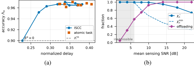
Fig. 4. ISCC effects: (a) accuracy–delay frontier swept over \beta^a , versus the atomic-task baseline; (b) optimal retention \chi_n^* , retention floor \chi_n^{\min} , and fraction of offloading UEs versus mean sensing SNR.
