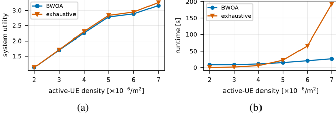
Fig. 2. Proposed BWOA matching versus exhaustive search, K = 3 , M^{u1} = 2 , M^{d1} = 1 : (a) attained utility, (b) runtime, versus active-UE density.
