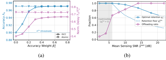
Fig. 4. ISCC effects: (a) accuracy–delay frontier swept over \beta^a , versus the atomic-task baseline; (b) optimal retention \chi_n^* , retention floor \chi_n^{\min} , and fraction of offloading UEs versus mean sensing SNR.
