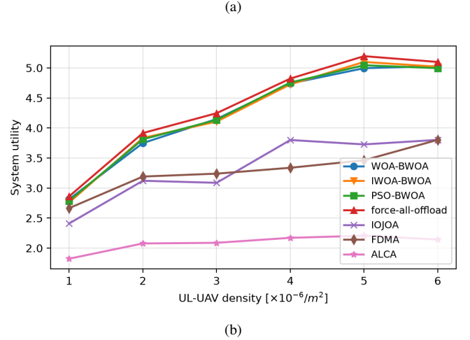
Fig. 3. (a) Utility versus active-UE density for WOA/IWOA/PSO-BWOA (MF-SIC), force-all-offload, IOJOA, FDMA, and ALCA. (b) Utility versus UL UAV-server density.
