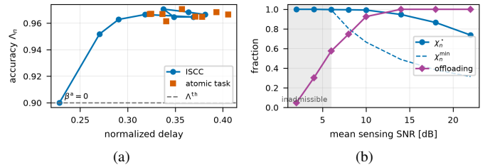
Fig. 4. ISCC effects: (a) accuracy–delay frontier swept over \beta^a , versus the atomic-task baseline; (b) optimal retention \chi_n^* , retention floor \chi_n^{\min} , and fraction of offloading UEs versus mean sensing SNR.
